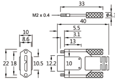
USB 3.0 Micro B
