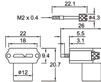
USB 3.0 Micro B - up
