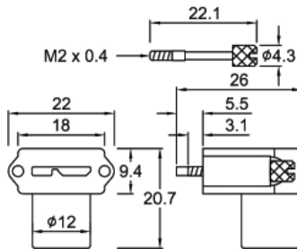
USB 3.0 Micro B - dw
